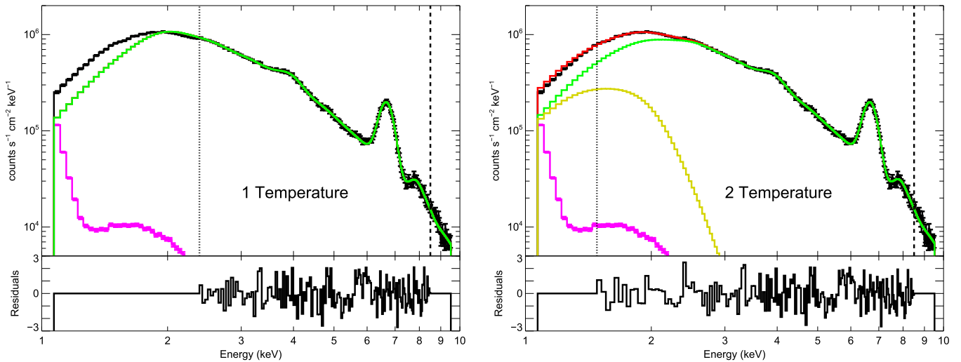
Figure 2. SAX background-subtracted count flux spectra (black histograms) and two model fits for the 14:56:30–15:01:29 UT period at the maximum of the 2007 June 1 flare with normalized residuals (the differences between the measured and best-fit fluxes as a fraction of the statistical 1\sigma uncertainties) shown below each spectrum. Left: 1-T (isothermal) function (green curve) fitted over the 2.3–8.5 keV energy range with T = 22 MK (1.9 keV), EM = 7.1 \times 10^{48} \text{ cm}^{-3} , and \chi^2_{\text{red}} = 1.21 ( \nu = 160 ). Right: 2-T (two-temperature) function (green and yellow curves with the red curve representing the sum of the two) fitted over the 1.5–8.5 keV energy range with T_1 = 22 MK (1.9 keV), T_2 = 2.9 MK (0.25 keV), EM_1 = 7.6 \times 10^{48} \text{ cm}^{-3} , EM_2 = 4.3 \times 10^{49} \text{ cm}^{-3} , and \chi^2_{\text{red}} = 1.18 ( \nu = 175 ). The same pre-flare background spectrum is shown in pink in both plots.
