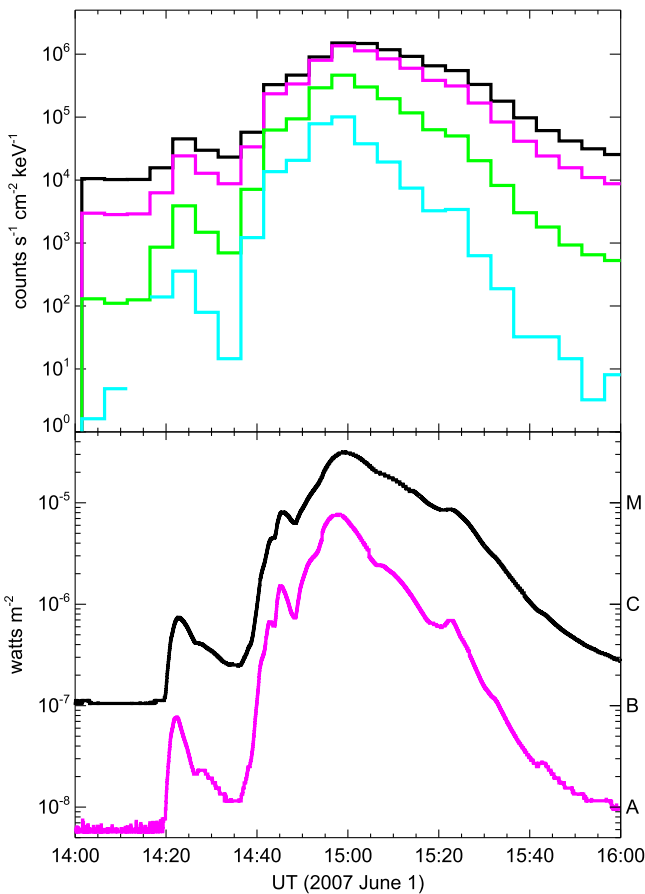
Figure 1. SAX and GOES light curves for the M2.8 flare on 2007 June 1. Top panel: SAX light curves plotted with 300 s time bins in four energy bands: 1.3–2 keV (black), 2–3.2 keV (pink), 3.2–5.3 keV (green), 5.3–8.5 keV (cyan). Bottom panel: GOES X-ray light curves at 1–8 Å (black) and 0.5–4 Å (pink) with 3 s time bins.
